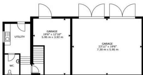
GARAGE FIRST FLOOR
